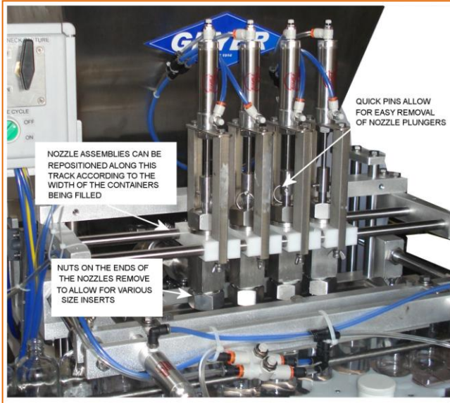
Adjustable Nozzle Assembly
