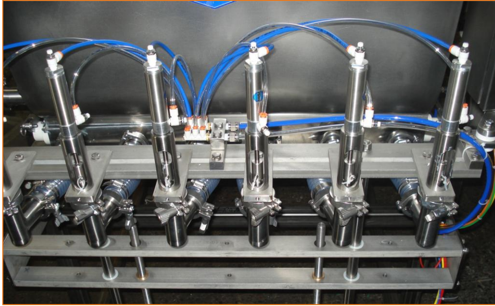
Positive Cut-Off Filling Nozzles
