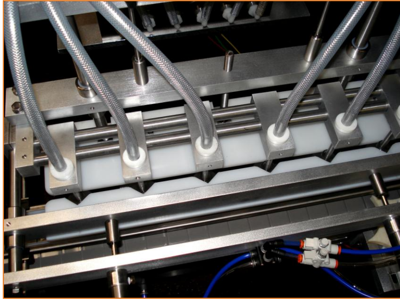
Container neck capturing mechanism
