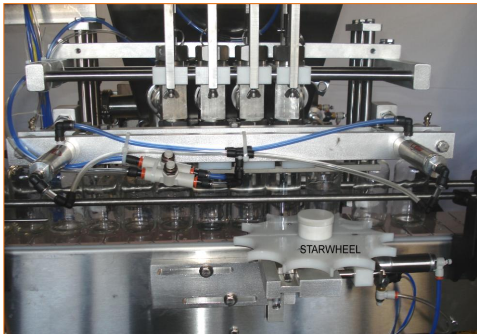
Starwheel Container Indexing Mechanism
