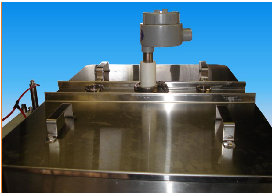
Hopper Lid with Level Control
