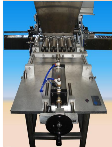
Piston Drive with Micro-Fill Adjustment
