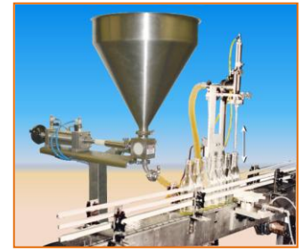
Diving nozzle mechanism
